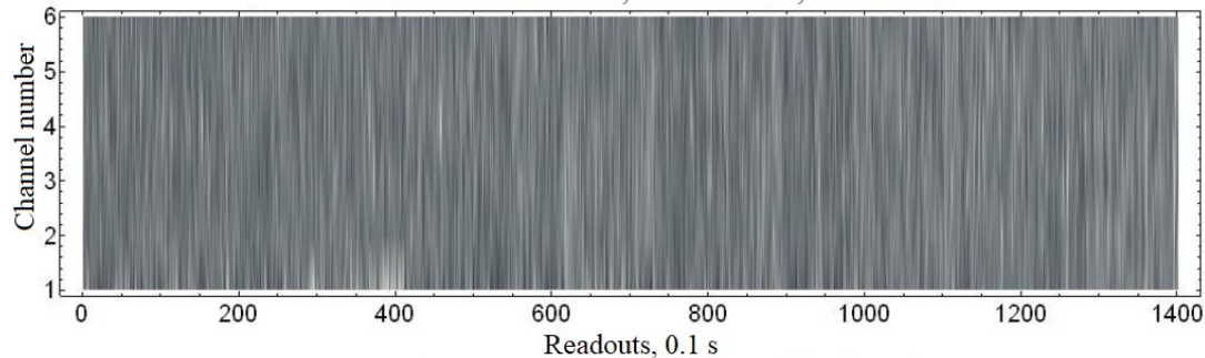
Total pulse, DM = 203 pc/cm 3
