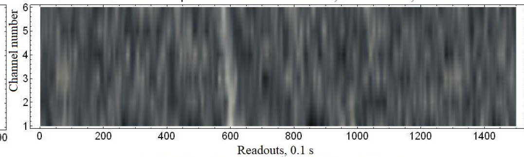
Total pulse, DM = 203 pc/cm 3 , SNR = 10.1
