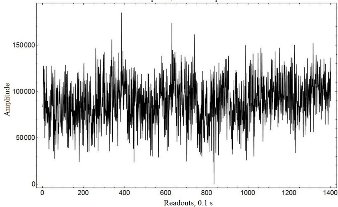
Total pulse, DM = 203 pc/cm 3
