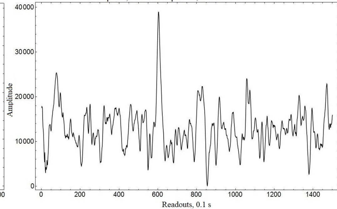
Total pulse, DM = 203 pc/cm 3 , SNR = 10.1
